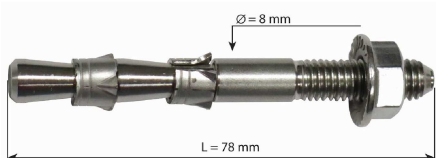
Art. 122 Hang Fix Ø 8 mm
