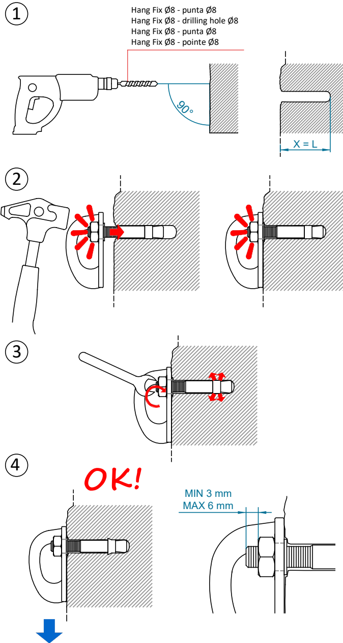
Art. 122 Hang Fix Ø 8 mm
