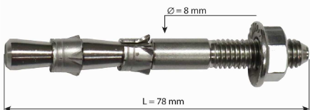
Art. 122 Hang Fix Ø 8 mm
